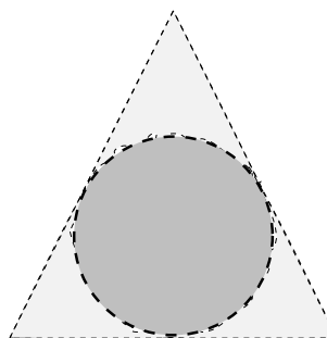
A = \text{an open disk inside } X
