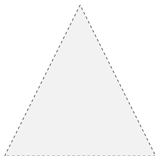
X = \text{an open triangle}
